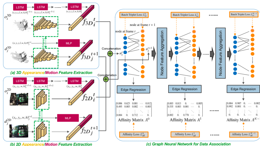
Fig. 2. Proposed Network.
