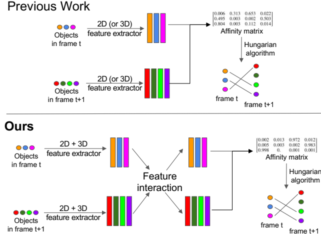
Fig. 1. (Top): Prior work often employs a 2D or 3D feature extractor and obtain the feature independently from each object. (Bottom): Our work proposes a joint 2D and 3D feature extractor and a feature interaction mechanism to improve the discriminative feature learning for data association in MOT.
